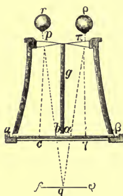
FIG. 205.—The refracting stereoscope of Brewster.
